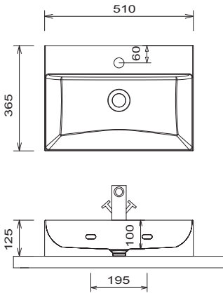
WMS 2305 61 (Straight) WTA 5136 1 (Orlando) SET FG60 09/10 WTA 3039 1 (Piccolo)
