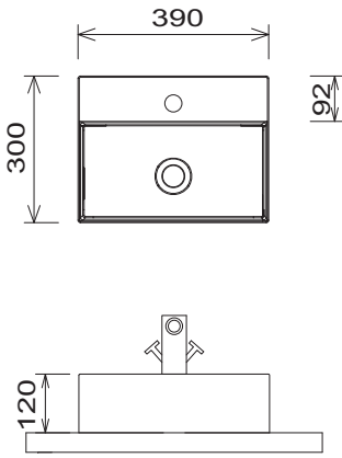
WMS 2305 61 (Straight) WTA 5136 1 (Orlando) SET FG60 09/10 WTA 3039 1 (Piccolo)
