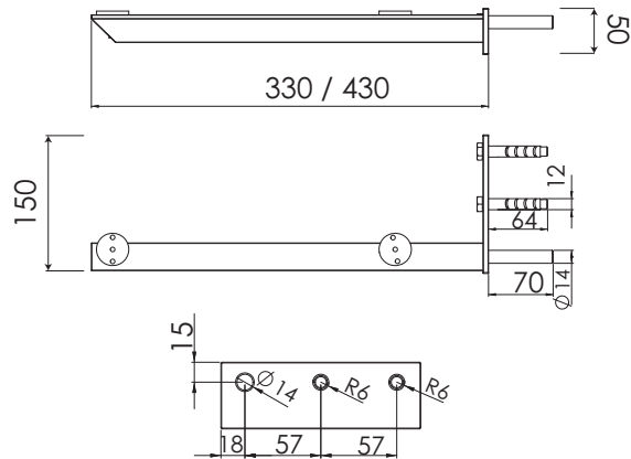
Console for washbasin tops PZ 1244 50/40
