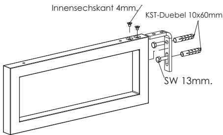
Towel holder console PZ 1133 49/40 & PZ 1233 49/40
