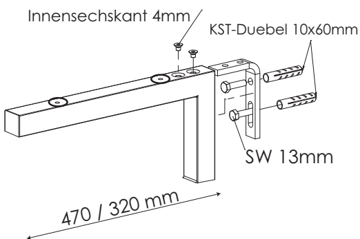
L-Console for washbasin tops PZ 1118 49/40 & PZ 1218 49/40
