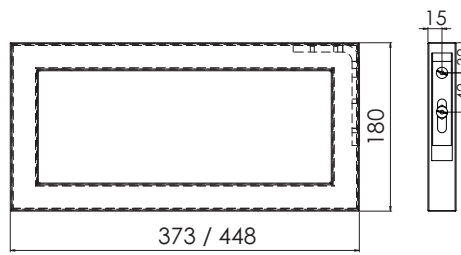
Towel holder console PZ 1133 49/40 & PZ 1233 49/40
