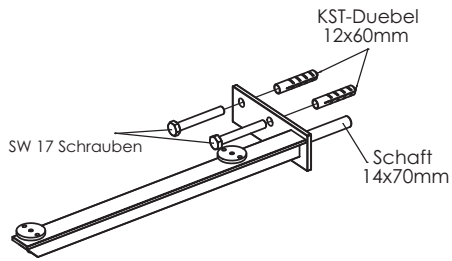
Console for washbasin tops PZ 1244 50/40
